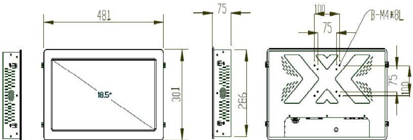
CUT OUT DIMENSION (468*288mm ) UNIT:mm
