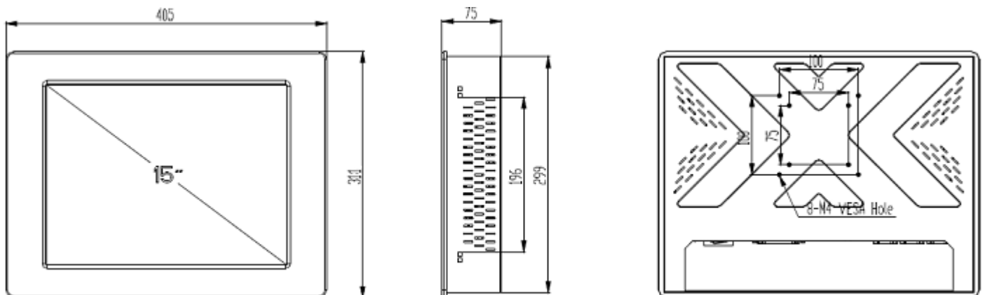
CUT OUT DIMENSION (395x301mm) UNIT:mm
